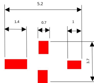
PCB Footprint
