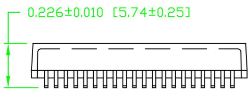
WITHOUT STANDOFF
