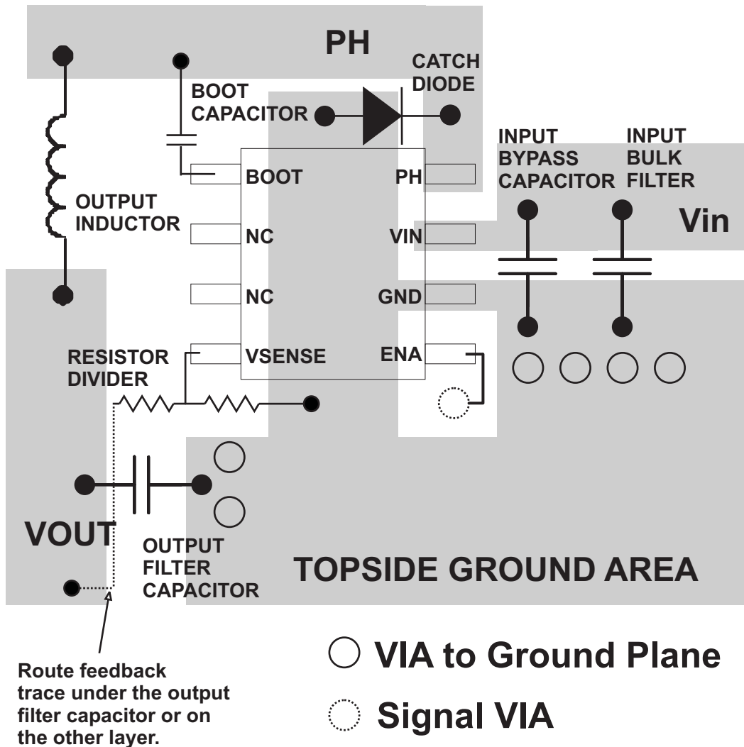
Figure 9. Design Layout
