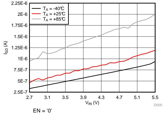
Figure 6. Shutdown Current
