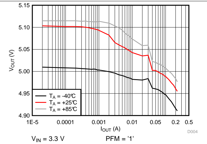
Figure 4. Load Regulation
