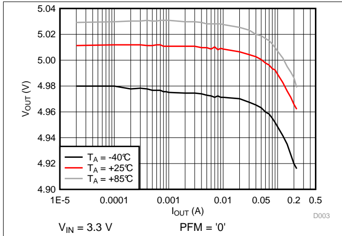
Figure 3. Load Regulation
