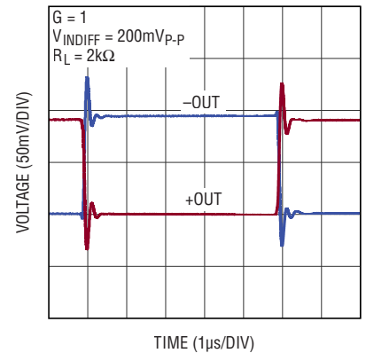
Small Signal Step Response
