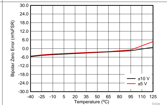
Figure 12. VOUT Bipolar Zero Error vs Temperature
