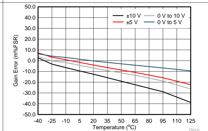
Figure 14. VOUT Gain Error vs Temperature
