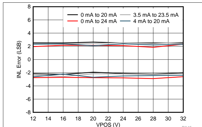
Figure 50. IOUT Unipolar Ranges INL vs VPOS
