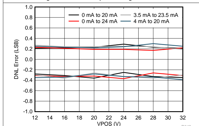
Figure 52. IOUT Unipolar Ranges DNL vs VPOS
