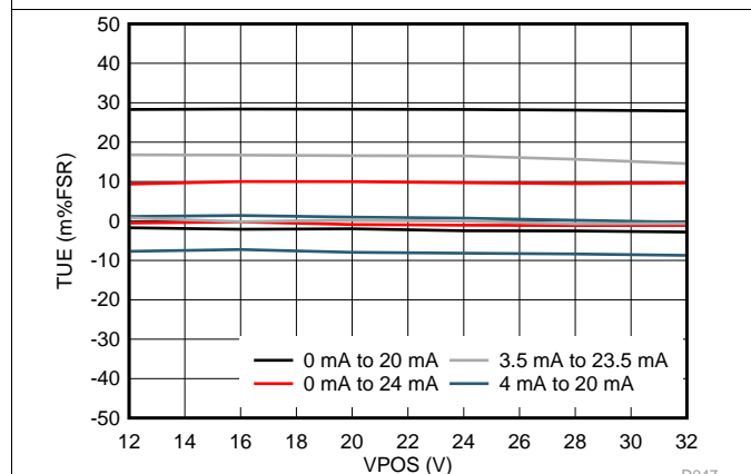
Figure 54. IOUT Unipolar Ranges TUE vs VPOS
