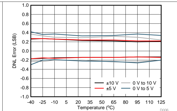
Figure 10. VOUT DNL vs Temperature
