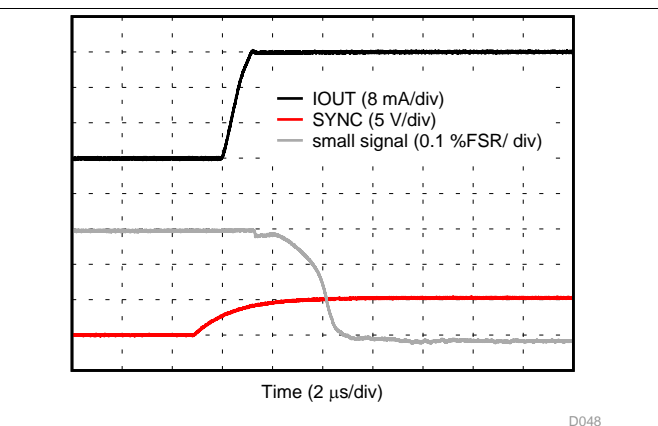
Figure 55. IOUT Settling Time, Rising Signal
