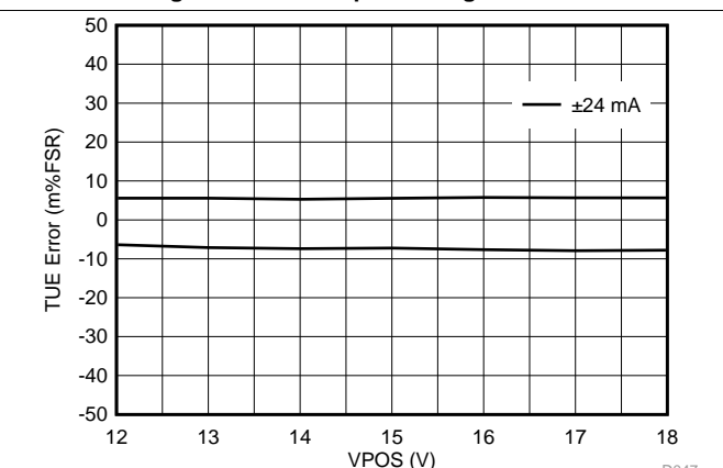
Figure 53. IOUT Bipolar Range TUE vs VPOS
