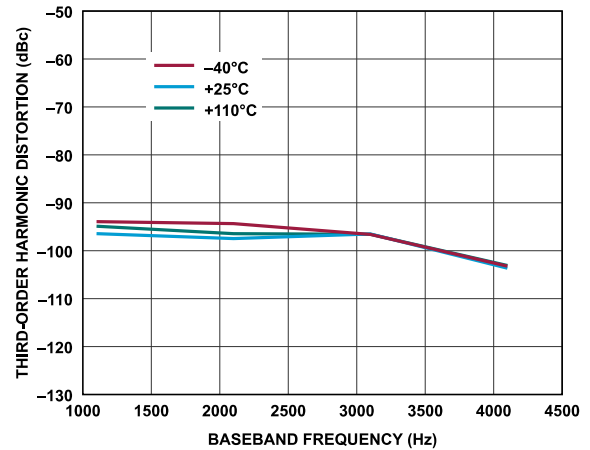
Figure 248. Receiver Third-Order Harmonic Distortion vs. Baseband Frequency, Gain Index = 255, ADC = Low Power
