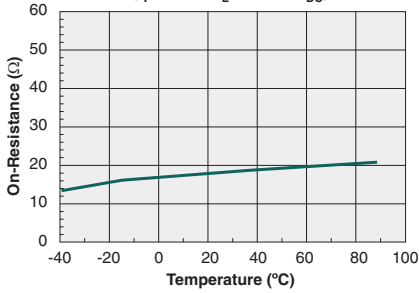
Typical On-Resistance vs. Temperature ( I_F=2mA , I_L=120mA_{DC} )
