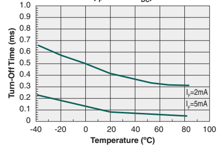
Typical Turn-Off Time vs. Temperature ( I_F=120mA_{DC} )
