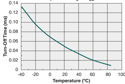
Typical Turn-Off Time vs. Temperature ( I_F=10mA, I_L=1A_{DC} )
