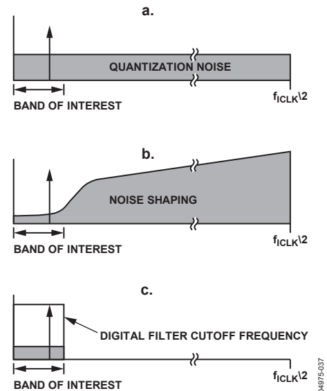
Figure 40. \Sigma - \Delta ADC
