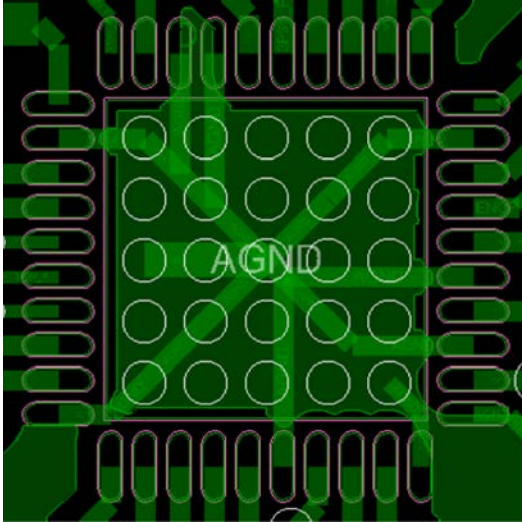
Figure 56. Evaluation Board Layout for the ADRF6720 Package
