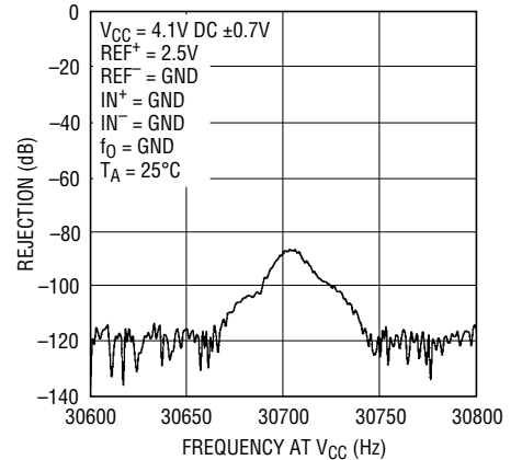
PSRR vs Frequency at V_{CC} (2x Speed Mode)
