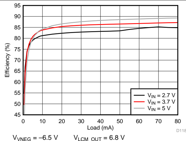
Figure 132. VNEG Efficiency
