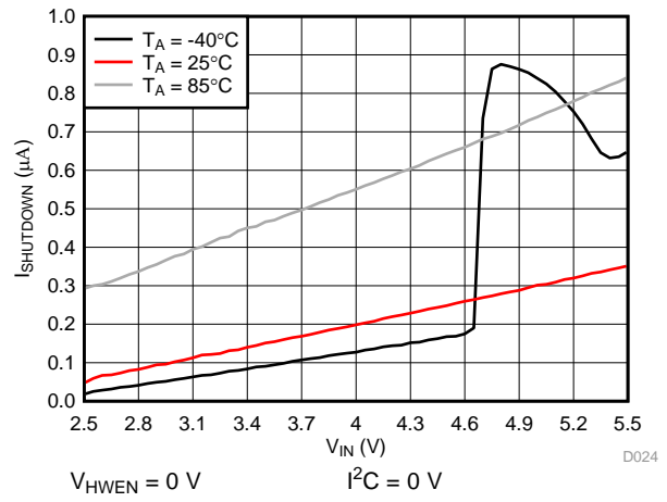
Figure 27. I_q Shutdown
