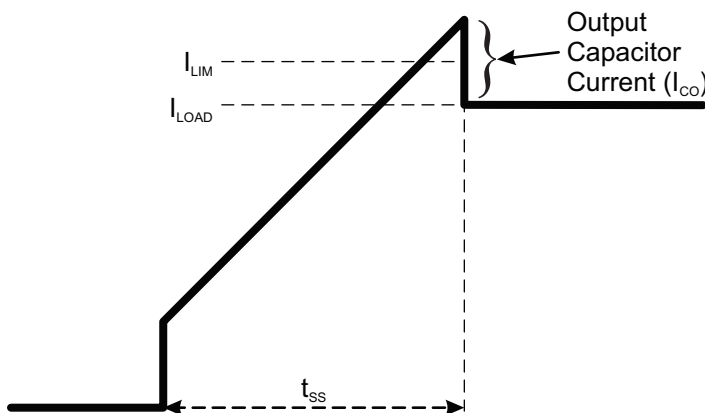
Figure 6: Output Current ( I_{CO} ) During Startup
