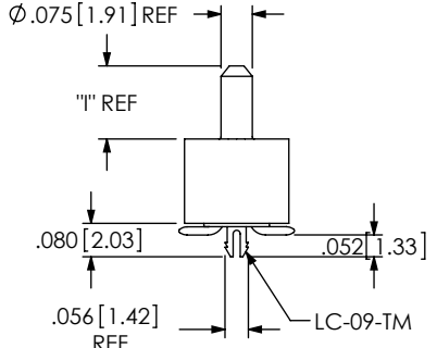
FIG 9 -EP-LC (DIFFERENT AS SHOWN, OTHERWISE SAME AS FIG 1)
