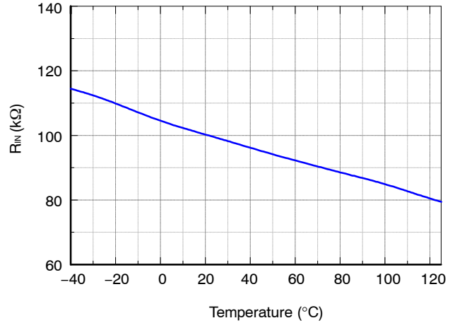
Figure 19. Input Pull-Down Resistance vs. Temperature
