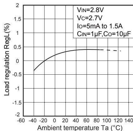
Fig.9 Load Regulation vs. Ambient Temperature (PQ018ENAHZPH)
