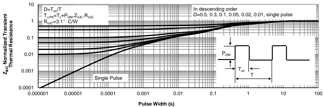
Figure 15: Normalized Maximum Transient Thermal Impedance for AOTF12N65L (Note F)
