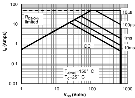
Figure 9: Maximum Forward Biased Safe Operating Area for AOT(B)12N65(L) (Note F)
