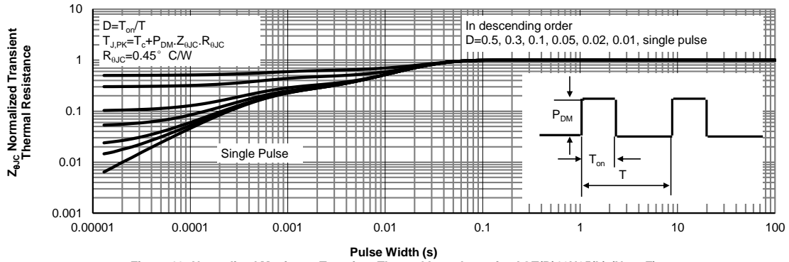
Figure 13: Normalized Maximum Transient Thermal Impedance for AOT(B)12N65(L) (Note F)
