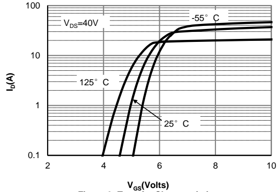
Figure 2: Transfer Characteristics
