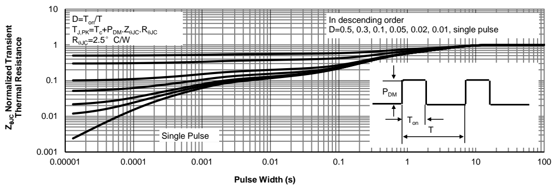
Figure 14: Normalized Maximum Transient Thermal Impedance for AOTF12N65 (Note F)
