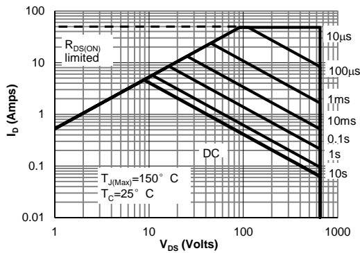
Figure 11: Maximum Forward Biased Safe Operating Area for AOTF12N65L (Note F)
