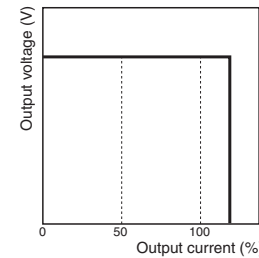
120-W/180-W/240-W/480-W Models
