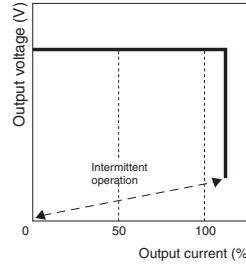
15-W/30-W Models
