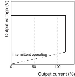
60-W/90-W Models
