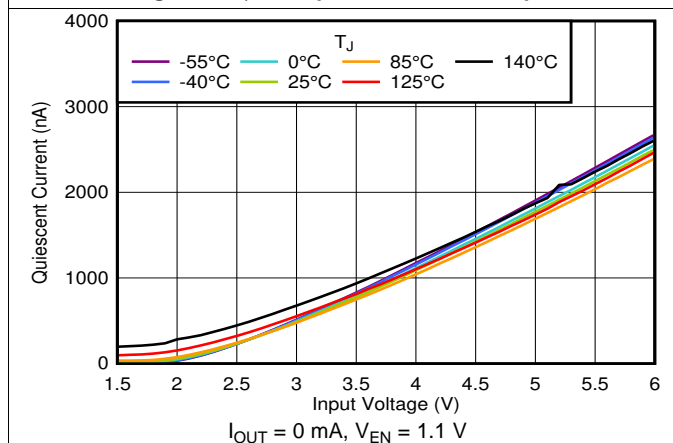
Figure 9. I_Q vs V_{IN} and Temperature
