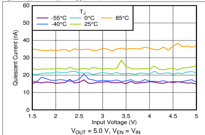
Figure 7. I_Q in Dropout vs V_{IN} and Temperature
