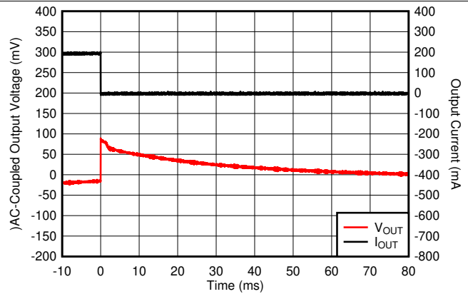
Figure 20. I_{OUT} Transient From 200 mA to 0 mA
