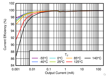
Figure 62. Current Efficiency vs I_{OUT} and Temperature
