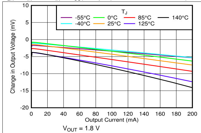
Figure 31. Load Regulation vs V_{IN} and Temperature
