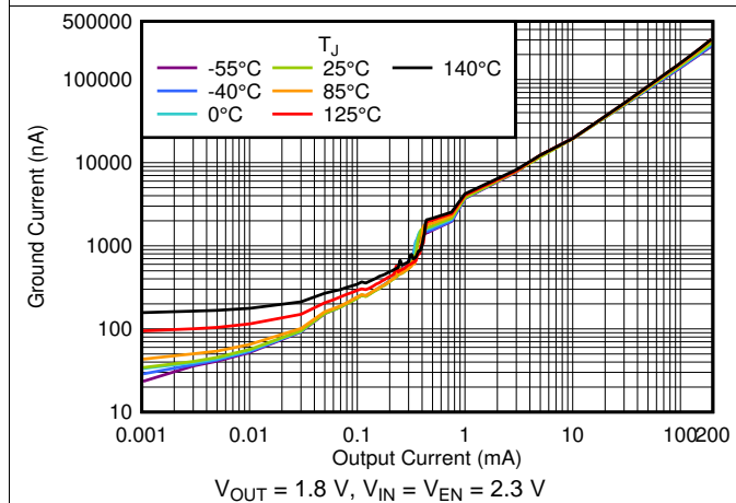
Figure 3. I_Q vs I_{OUT} and Temperature up to 200 mA
